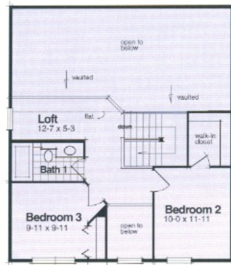
Standard Second Floor Plan
