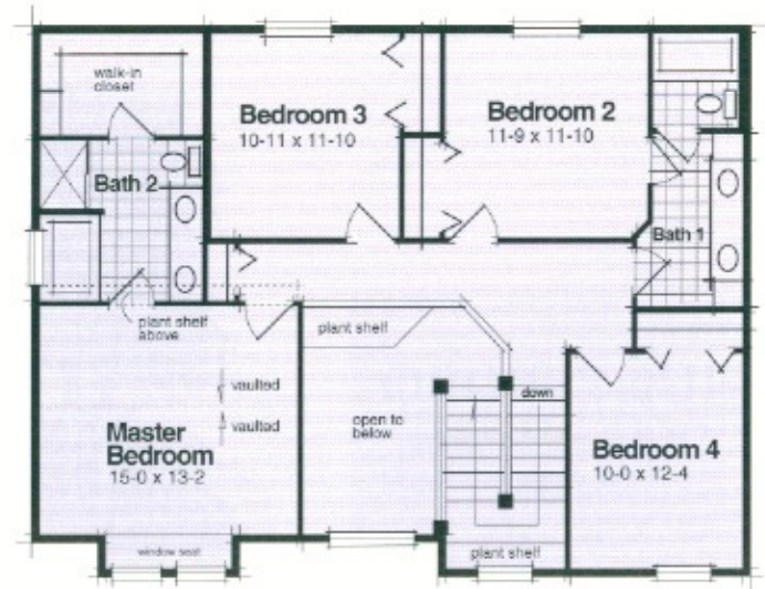
Standard Second Floor Plan
