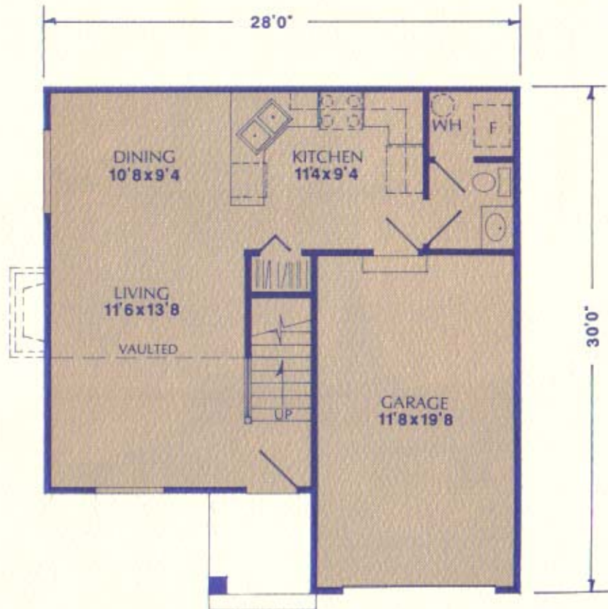
First Floor Layout 544 sq. ft.
