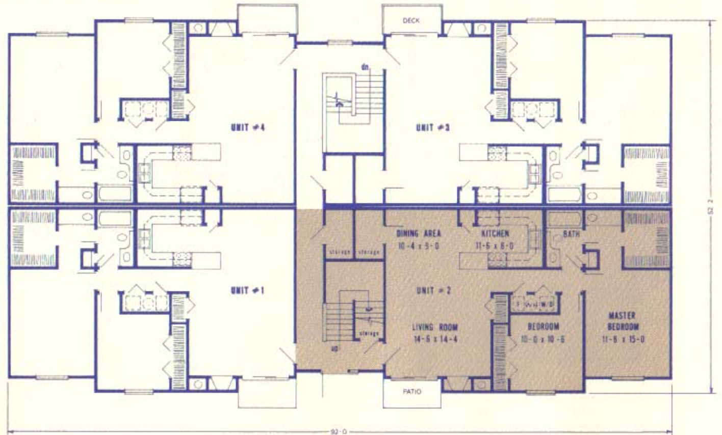
Floorplan and Hall Configuration for First Floor Unit Plan shown is for slab or crawlspace. Basement plan available.
