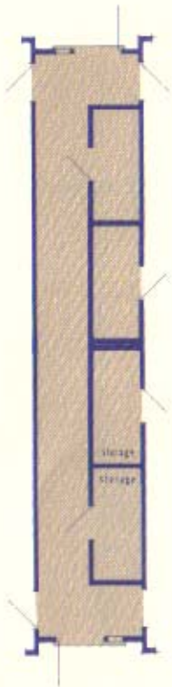
Hall Configuration for R510 4-Unit Plan (Ranch) Overall Length = 88'-0"
